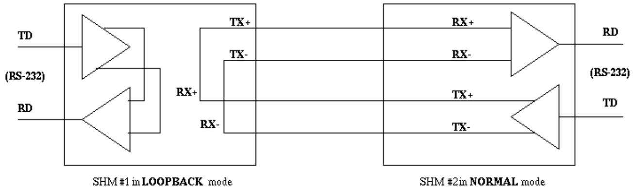
Figure 2: SHM-B Modem Test Configuration (Loopback Test)
