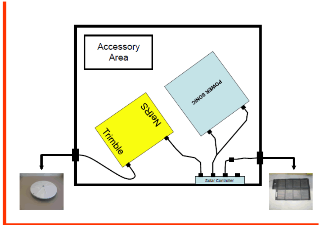
First Connect Battery. Ensure + Red, - Black!!!
