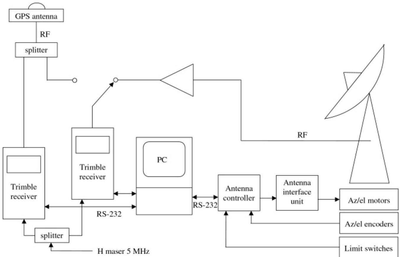
Block diagram of Antenna & Multipath Calibration System
